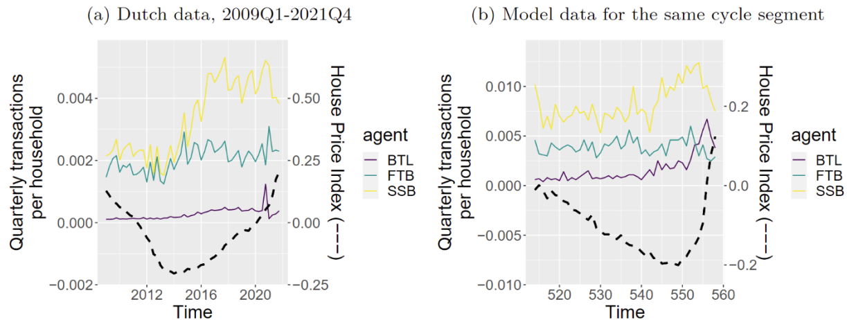
Figure B.3 Number of transactions per quarter for each owner type for the Netherlands (left panel) and in the model (right panel).
